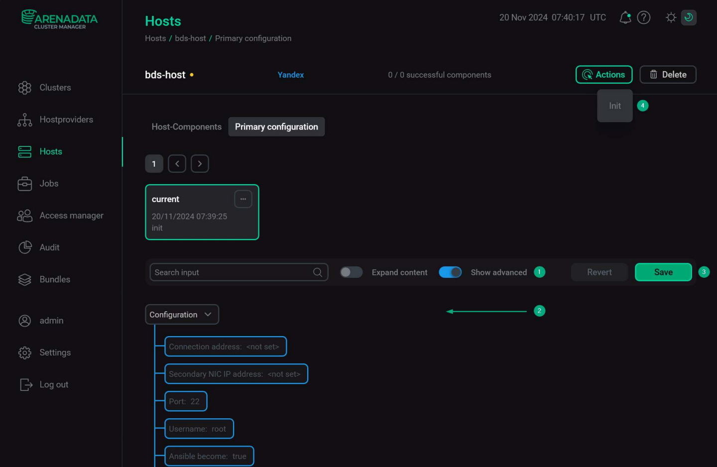
Go to configuring a host
