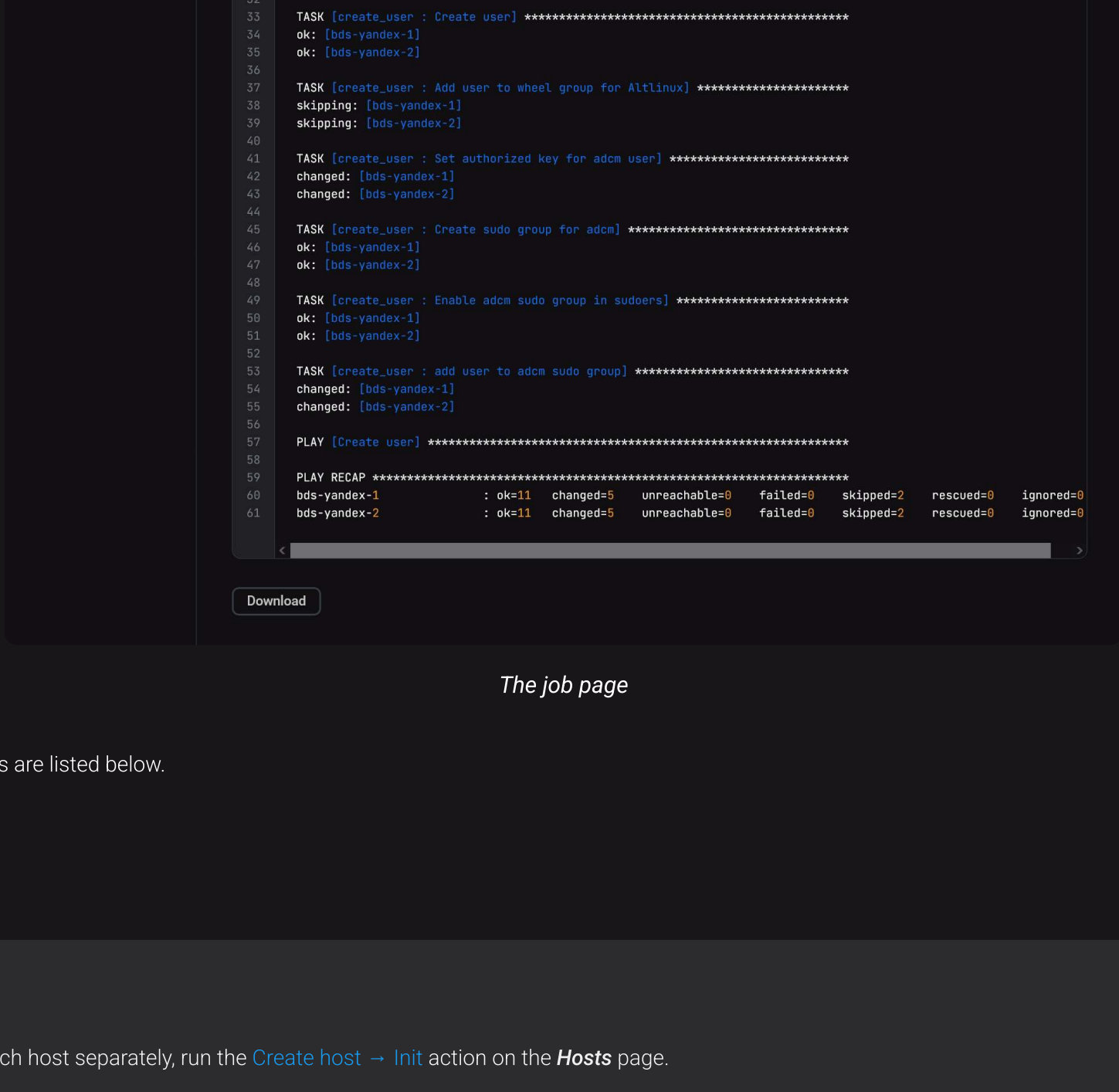
The job page
