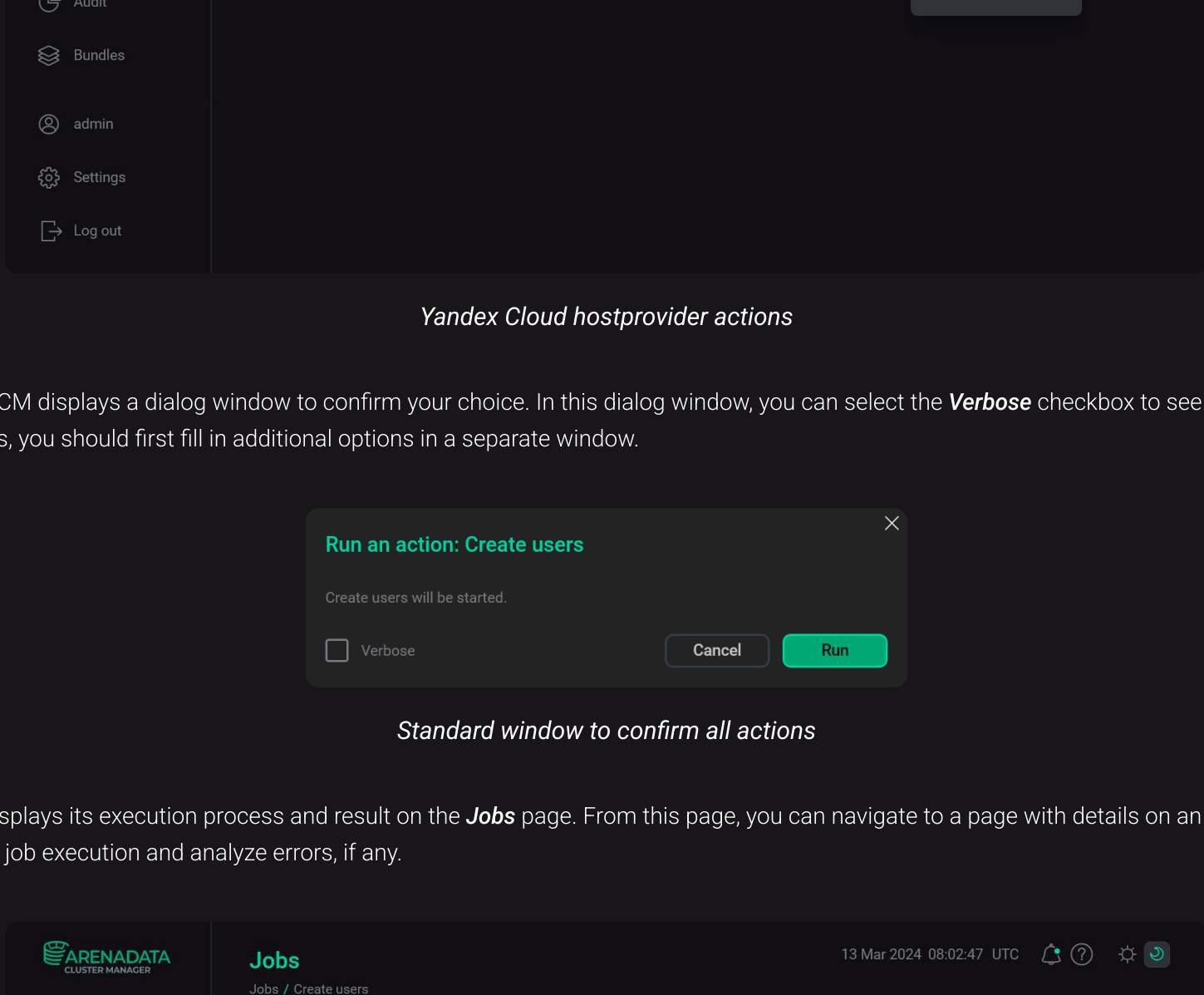
Yandex Cloud hostprovider actions
