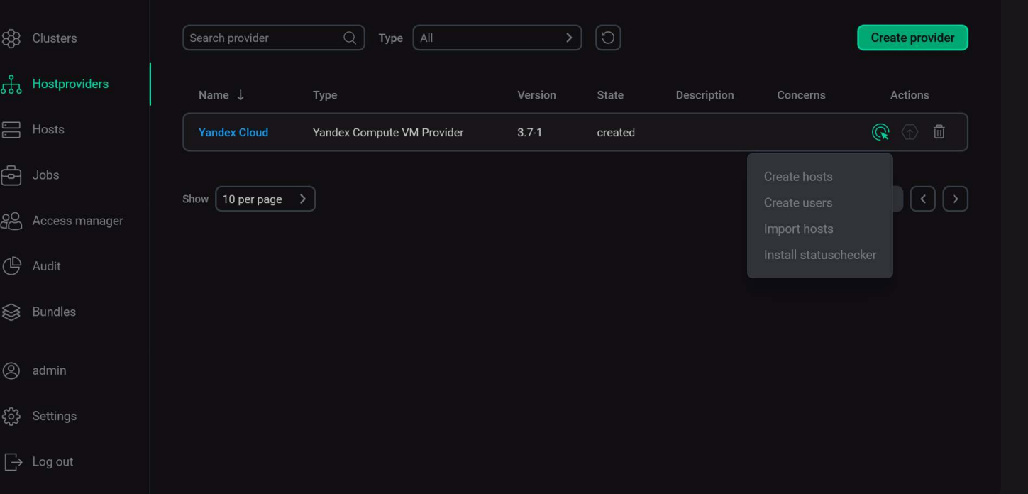
Find a subnet identifier
