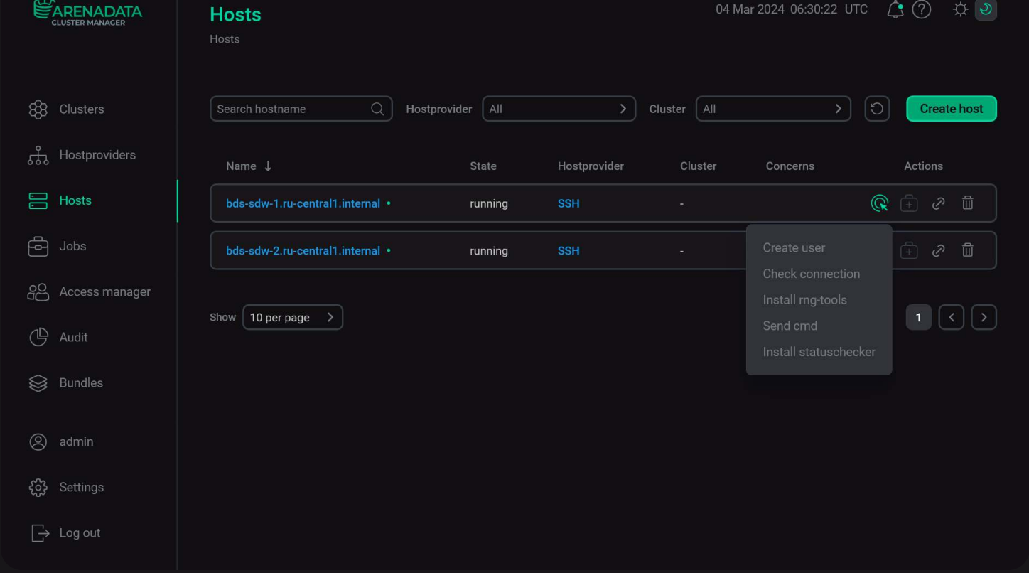
Host actions
